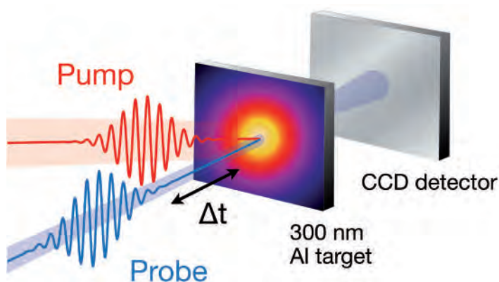
Figure 1 Schematic of the experiment: the FLASH pulse was split into two, with the first pulse creating a warm dense transient system and the second probing its free-free opacity in transmission.
