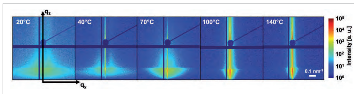
Figure 2 GISAXS pattern for small PMMA colloids deposited on the surface and annealed from room temperature up to 140°C.
