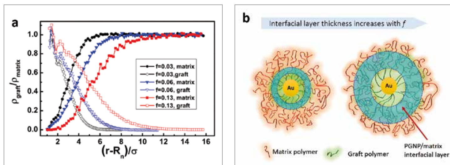
Figure 1 (a) Radial density profiles for graft and matrix monomers from the centre of nanoparticle for different f values (ratio of grafted to matrix chain length), calculated from MD simulation, where r , R_n and \sigma are the radial distance, radius of nanoparticles and size of a monomer respectively [2]. (b) Schematic of interfacial layer surrounding PGNP. The annular region represents the interfacial layer where matrix polymers penetrated into the graft polymer brushes.
