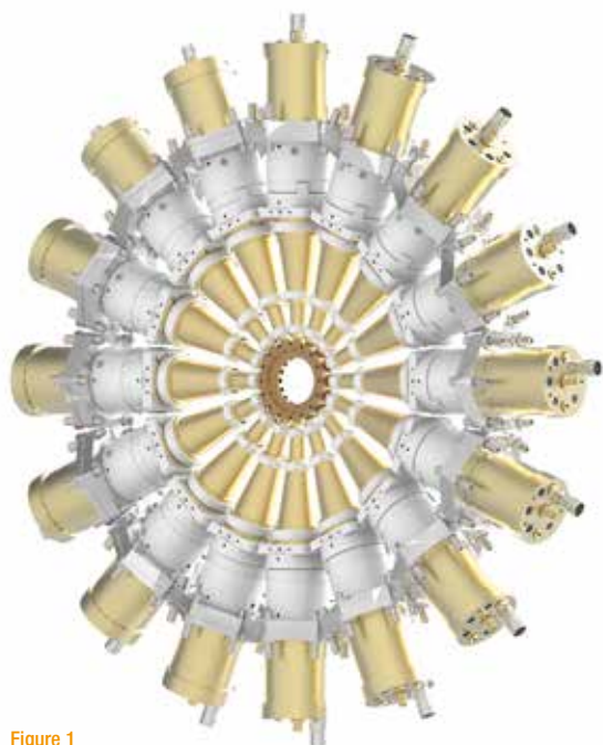
Figure 1 The employed angle-resolving spectrometer built at beamline P04 at DESY. Copyright Frank Scholz.
