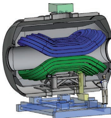
Figure 3 Conceptual design of the 200 t heavy dipole magnet for MADMAX, which will have an aperture of 1.35 m and provide a field of 8.9 T
