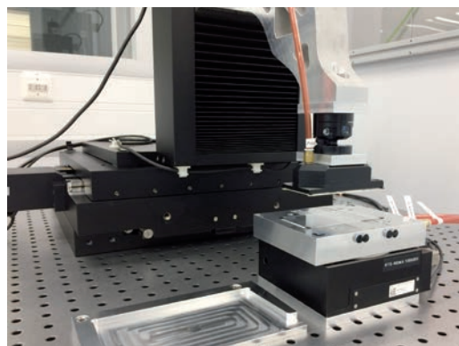
Figure 3 Automated pickup and positioning system for the CMS detector module assembly
