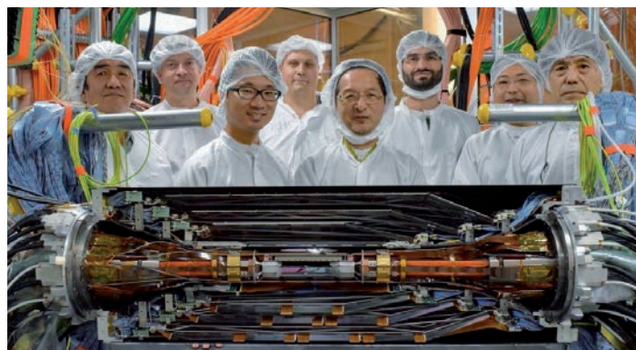
Ready for collisions: After insertion of the vertex detector, the research programme kicked off at Belle II.
