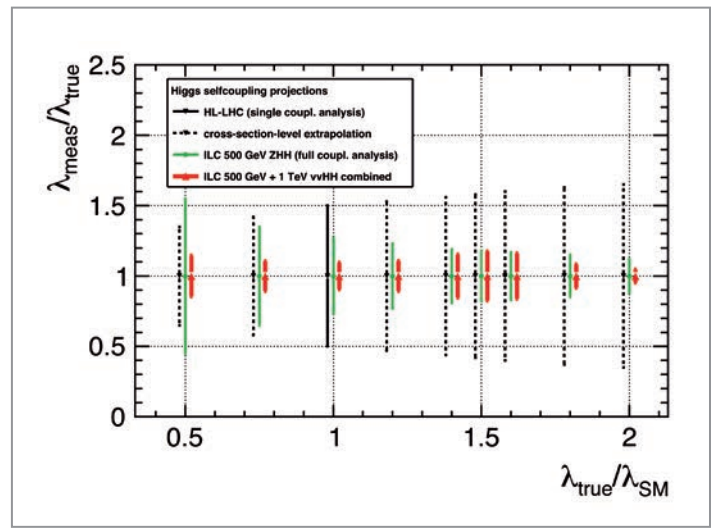
Figure 4 Prospects for the measurement of the Higgs self-coupling depending on its value (normalised to the SM prediction): The black error bars show a cross-section-level extrapolation of the HL-LHC projection, which only exists for the SM case. The green and red bars show the ILC projections at 500 GeV alone and combined with 1 TeV, respectively.
