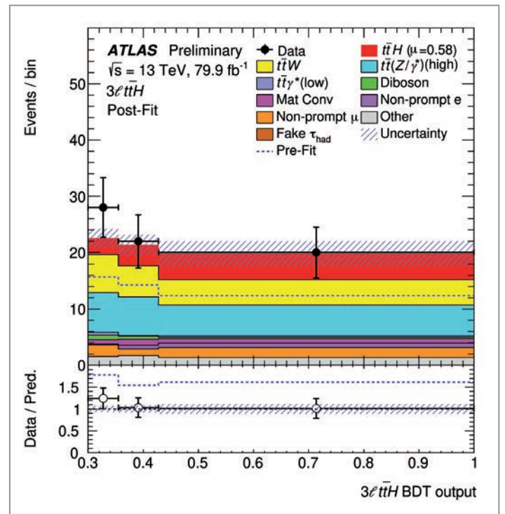
Figure 3 Distribution of the BDT output for events with three leptons (electrons or muons). The data are shown together with the fitted distributions from the t\bar{t}H signal (red) and the various backgrounds. The background from the t\bar{t}Z process is shown in light blue [1].
