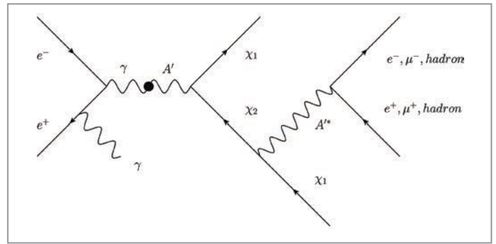
Figure 3 Feynman diagram for dark-photon A' production with A' decay into inelastic dark matter
