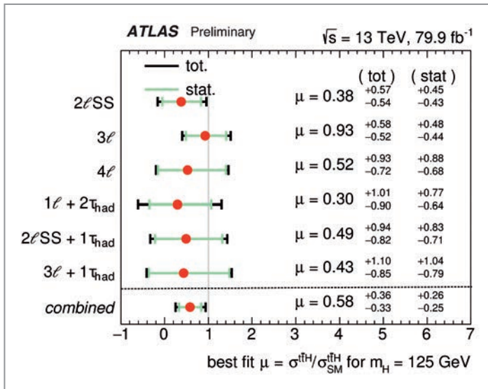
Figure 4 Observed best-fit values of the t\bar{t}H signal strength \mu and their uncertainties, separately for each analysis channel and in combination [1]
