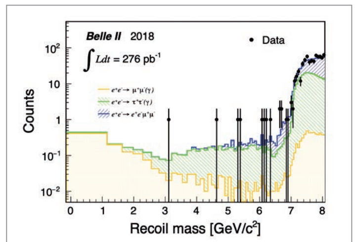
Figure 2 Recoil mass spectrum of the muon pair sample. Simulated samples (histograms) are rescaled for luminosity and corrected for efficiency. From [1].
