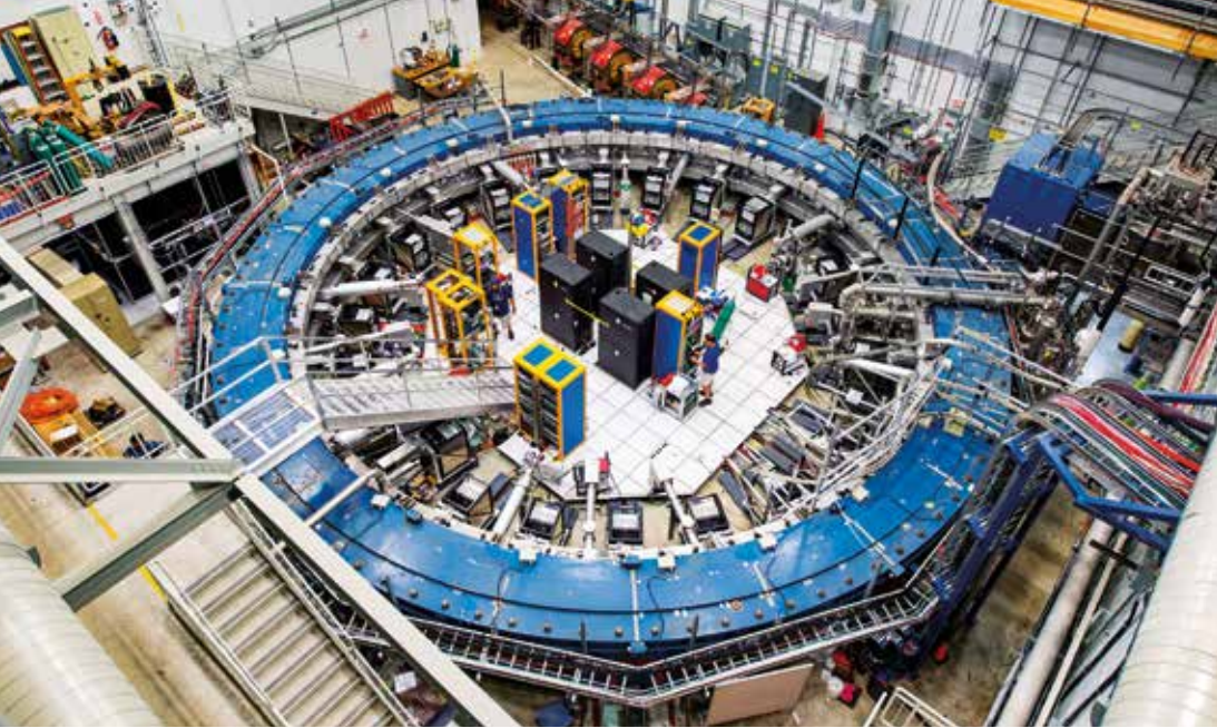
The Muon g-2 experiment operates at freezing temperatures of minus 267 degrees Celsius and observes how strongly muons oscillate in an external magnetic field.
